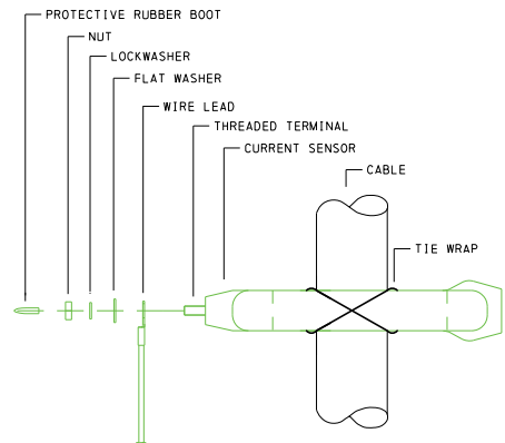
DETAIL B REAR VIEW CURRENT SENSOR MOUNTING
