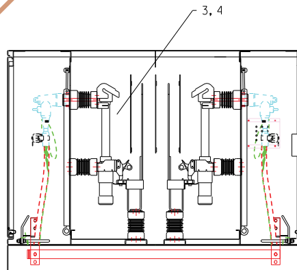
SME-4Z FUSE FITTED SECTION THROUGH DETAIL A-A (MSG-12)
