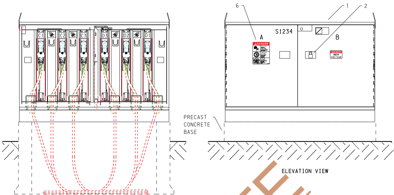
15T422DD*** (PMSG-200-9) & 15T421DD*** (PMSG-200-12) FUSE COMPARTMENT (C & D)
