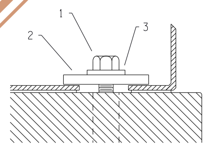
ANCHORING DETAIL (TYPICAL REAR)
