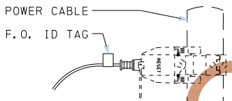
DETAIL E FOR INSTALLATION OF FAULT CURRENT INDICATOR WITH ELBOW CONNECTION REF.: 63 00 07 00 48 005 AND 63 00 07 00 48 006
