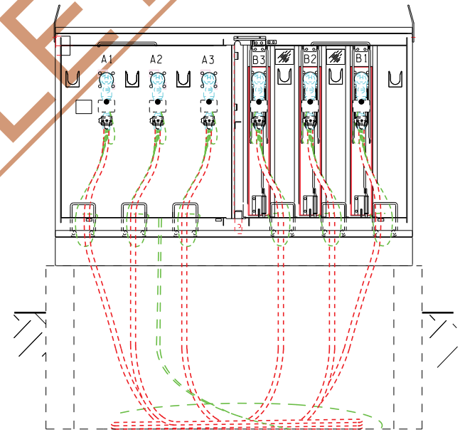
25T421DD*** (MSG-200-12) FEED THROUGH & FUSE COMPARTMENT ( A & B )
