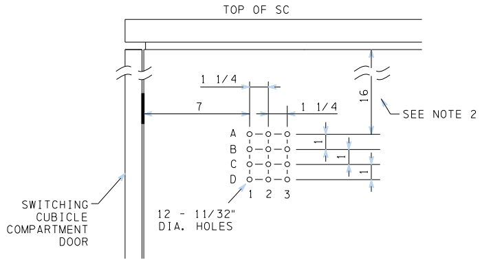
TYPICAL LED LOCATION
