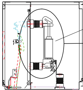
CLIP MOUNT FUSE FITTED SECTION THROUGH DETAIL A-A
