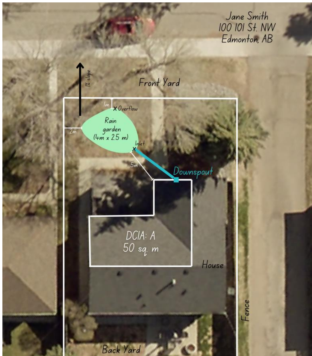
Figure 12: Sample computer generated project sketch
